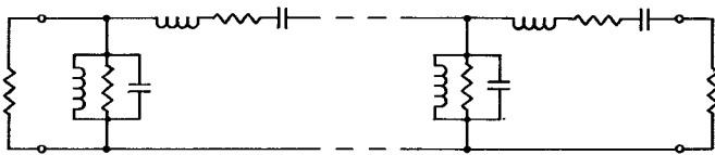
Fig. 3. Filter design example.
