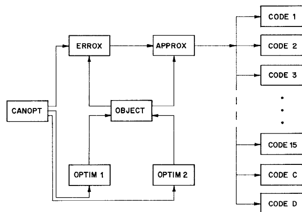
Fig. 2. The subprograms.
